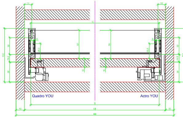
AVT YOU with Aluminum Profile
