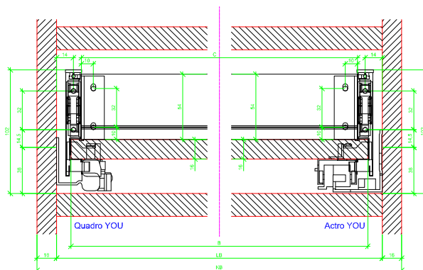
AVT YOU Rear Panel Connectors with Aluminum Profile
