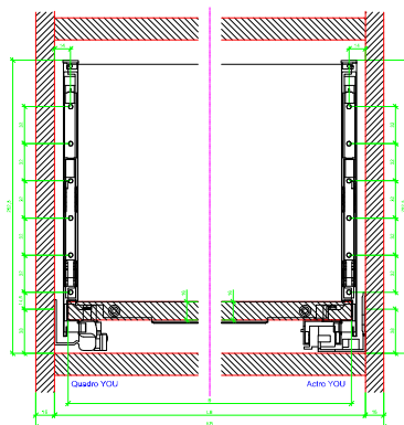
AVT YDU with Steel Rear Panel
