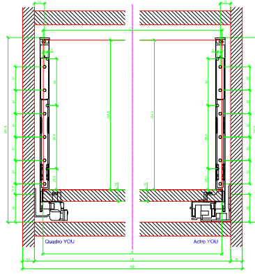
AVT YDU with Wooden Panel
