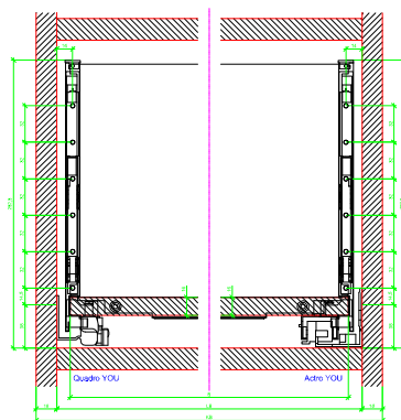
AVT YOU with Steel Rear Panel
