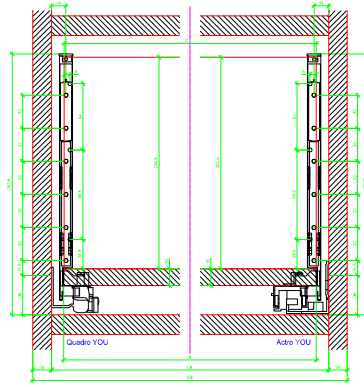
AVT YOU with Wooden Panel
