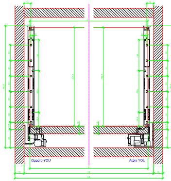
AVT YDU with Wooden Panel
