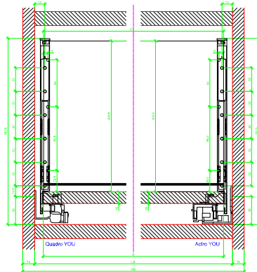
AVT YDU with Aluminum Profile
