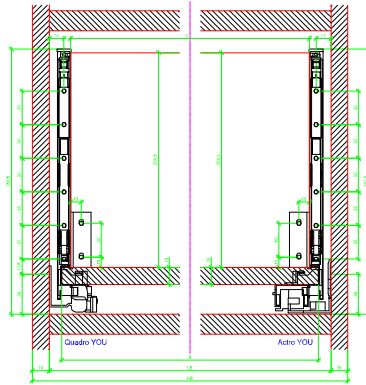
AVT YDU Rear Panel Connector with Wooden Panel
