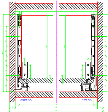
AVT YOU Rear Panel Connector with Wooden Panel
