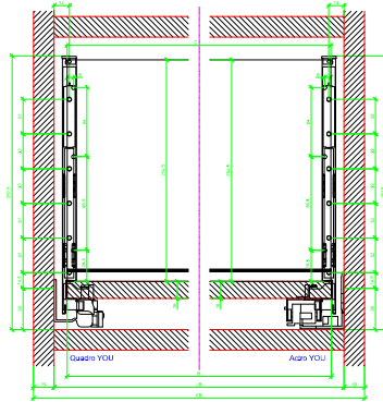
AVT YDU with Aluminum Profile
