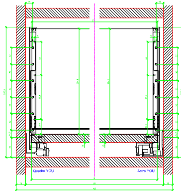
AVT YOU with Aluminum Profile
