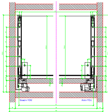
AVT YDU Rear Panel Connector with Aluminum Profile
